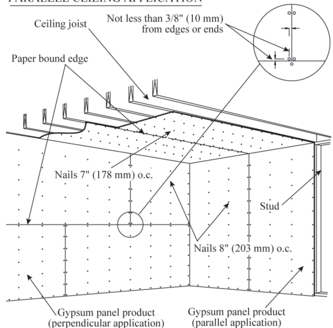
Figure 7 Double nailing
