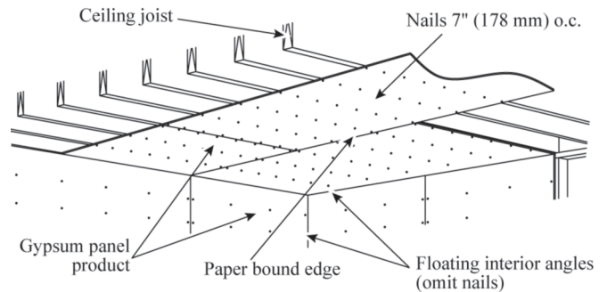
Figure 6 Single nailing
