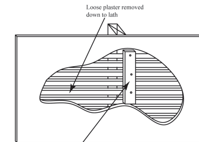
Figure 10 Shimmed plaster wall
