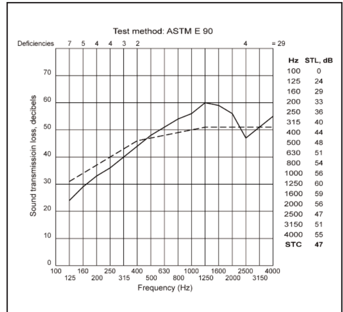
Figure 12 STL Curve
